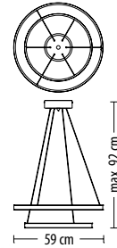
5319 Z-2 Q LED 57,4W 3780 lm* 230V
