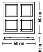
5363 PL-4 Q LED 53 W 3450 lm* 230V
