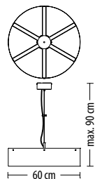
5540 Z-6 Q LED 27 W 2010 lm* 230 V
