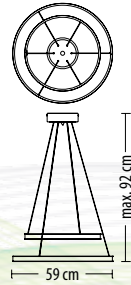
5318 Z-2 Q LED 57,4W 3780 lm* 230V
