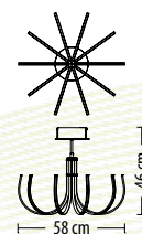
5025 Z-6 Q LED 39 W 2940 lm* 230 V
