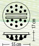
5476 PL-2 Q LED 16,5 W 1260 lm* 230 V
