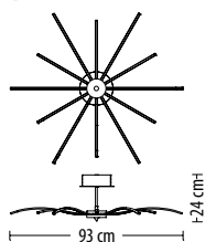
5024 PL-12 Q LED 40 W 3020 lm* 230 V
