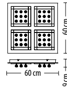
5362 PL-4 Q LED 52,5W 3450 lm* 230V
