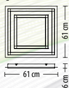
5369 PL-2 Q LED 59 W 3880 lm* 230 V
