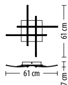
5242 PL-4 Q LED 17,3 W 1340 lm* 230 V
