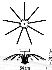
5240 Z-9 Q LED 41 W 3020 lm* 230V
