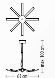
5581 Z-8 Q LED 35W 2680 lm* 230V
