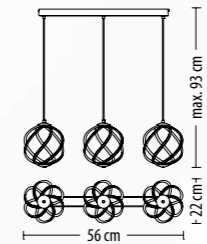
5392 Z-3 Q LED 60 W 3870 lm* 230V
