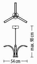
5644**** Z-3 Q LED 32,8W 2520 lm* 230V
