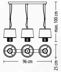
5750 Z-3 Q LED 34,4W 2640 lm* 230V
