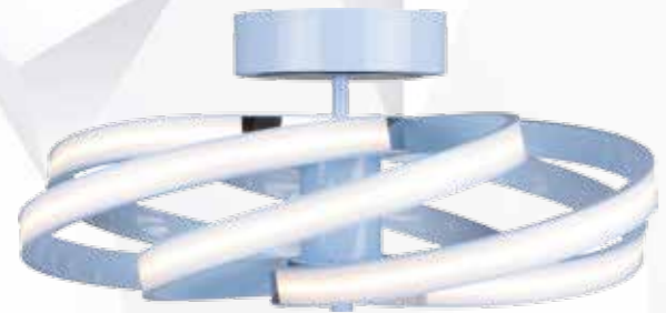
5651 PL-6 Q LED 57,3W 4410 lm* 230V
