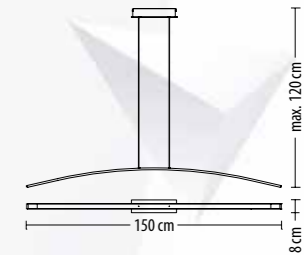
5304 Z-1 Q LED 25W 1675 lm* 230V
