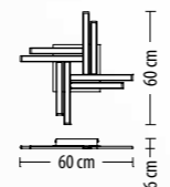
5316 PL-8 Q LED 44 W 3360 lm* 230 V
