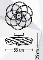
5651 PL-6 Q LED 57,3W 4410 lm* 230V
