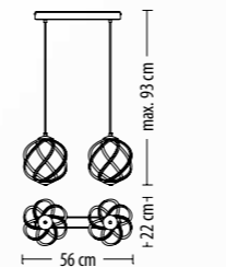
5393 Z-2 Q LED 40 W 2580 lm* 230V
