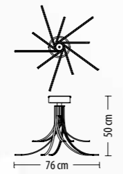
5440 Z-12 Q LED 60W 4530 lm* 230V
