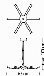
5583 Z-6 Q LED 26 W 2000 lm* 230 V
