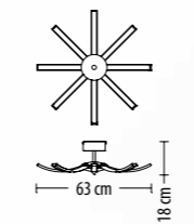
5585 PL-8 Q LED 35W 2680 lm* 230V
