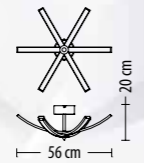
5573 PL -6 Q LED 30W 2260 lm* 230V
