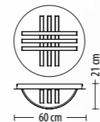
5471 PL-6 Q LED 54 W 4150 lm* 230 V
