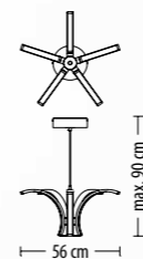
5642**** Z-5 Q LED 54,6W 4200 lm* 230V
