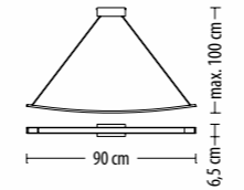
5406 Z-1 Q LED 21,9W 1680 lm* 230V
