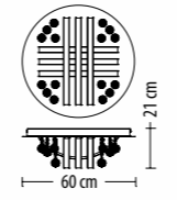
5470 PL-6 Q LED 54 W 4150 lm* 230 V
