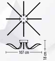
5258 PL-8 Q LED 35 W 2680 lm* 230V
