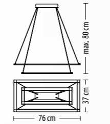
5344 Z-2 Q LED 59 W 3880 lm* 230 V
