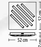
5502 PL-5 Ø LED 35,5 W 2730 lm* 230 V
