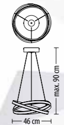
5670 Z-3 Q LED 53,3W 4095lm* 230V
