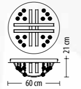
5473 PL-4 Q LED 36 W 2770 lm* 230 V
