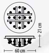
5472 PL-4 Q LED 36 W 2770 lm* 230 V
