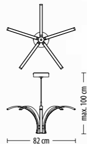
5640** Z-5 Q LED 41W 3150 lm* 230V
