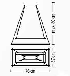
5345 Z-2 Q LED 59 W 3880 lm* 230 V
