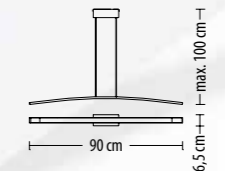
5405 Z-1 Q LED 21,9W 1680 lm* 230V
