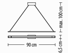
5407 Z-1 Q LED 21,9W 1680 lm* 230V
