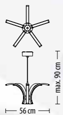
5643** Z-5 Q LED 27,3W 2100 lm* 230V
