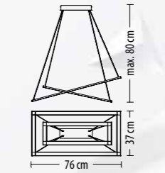
5346 Z-2 Q LED 59 W 3880 lm* 230 V
