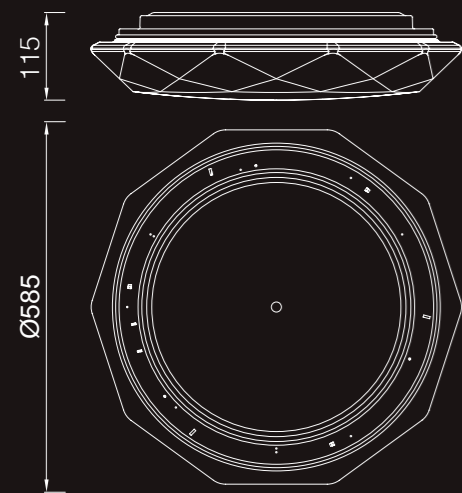
REF.3679 55W LED 55W 3000K-6500K 4200lm 220-240V
