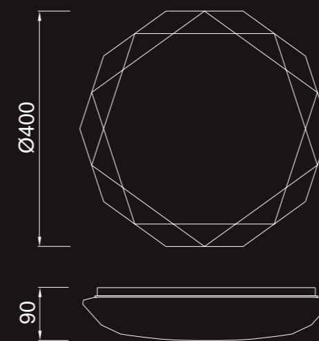
REF.5938 24W LED 24W 3000K-6500K 1400lm 220-240V
