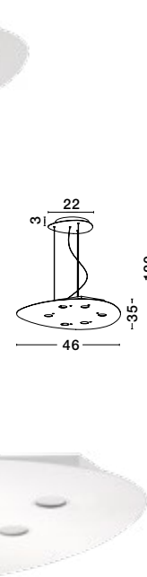
Triangolo 51609201 Aluminium Sand White LED 30 Watt 230 Volt 1800Lm 3000K IP20 L: 46 W: 45.5 H: 120 cm
