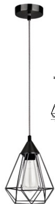
new Paolo 7605180 Black Metal Black & White Fabric Wire E27 1x40 Watt 230 Volt IP20 Bulb Excluded D: 17 H: 22.5 H2: 120 cm BULB EXCL. A++ E
