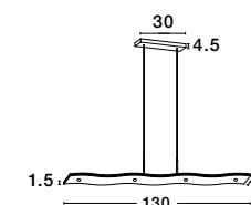
Fuori 51611001 Aluminium Sand White Dimmable LED 40 Watt 230 Volt 2400Lm 3000K IP20 L: 130 W: 8 H: 130 cm
